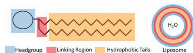
Figure 2. Generic lipid and lipid vesicle (liposome) structures.
