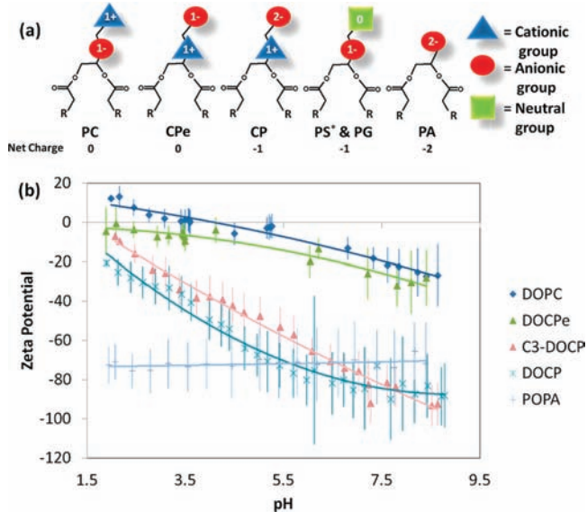
Figure 3. (a) Illustration of the charge orientation and net charge of naturally occurring phospholipid headgroups (PC, PS, PG, PA) and the CP lipid headgroups (CPe and CP). *The neutral block of the PS headgroup contains a primary amine and carboxylate that are zwitter-neutral at physiological pH. (b) Liposome zeta-potential as a function of solution pH.
