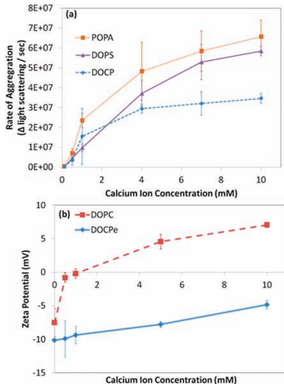
Figure 4. (a) Calcium-induced liposome aggregation rates. (b) Shift in zeta potential in the presence of \text{Ca}^{2+} .
